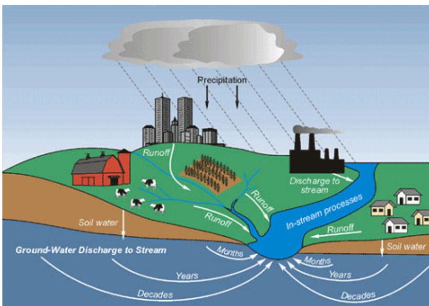
Figure 3.1: Model of the Water Cycle
